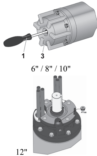
Figure 5-5: Checking the motor fluid
