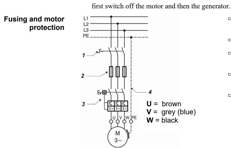
Figure 5-10: Fusing and motor protection
