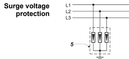
Figure 5-12: Surge voltage protection
